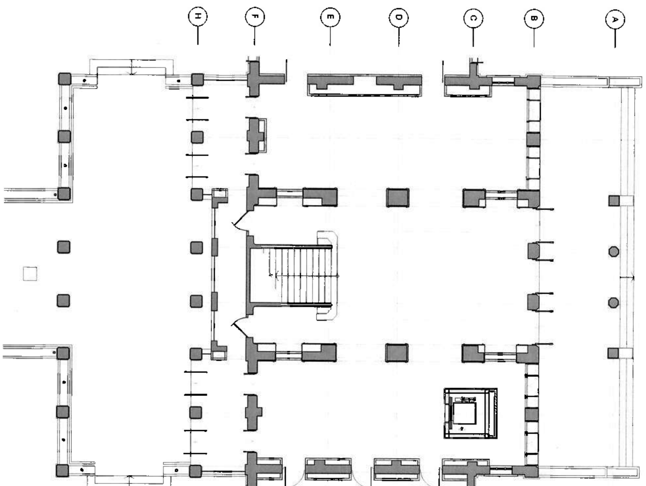
4 1st FLOOR DOOR & WINDOW PLAN SCALE 1:100
