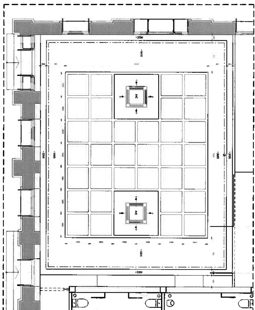
CEILING LIGHTING & AIR CONDITION LAYOUT SCALE 1:50
