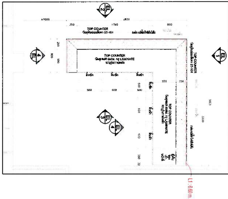
PLAN (FB08 / FB09 DETAIL) SCALE 1:25
