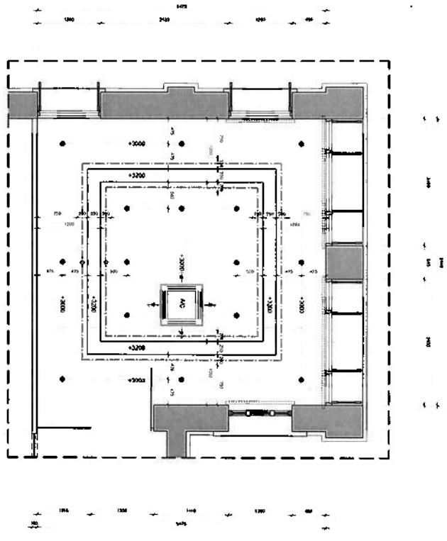
Fig. 2 CEILING & LIGHTING LAYOUT SCALE 1:50
