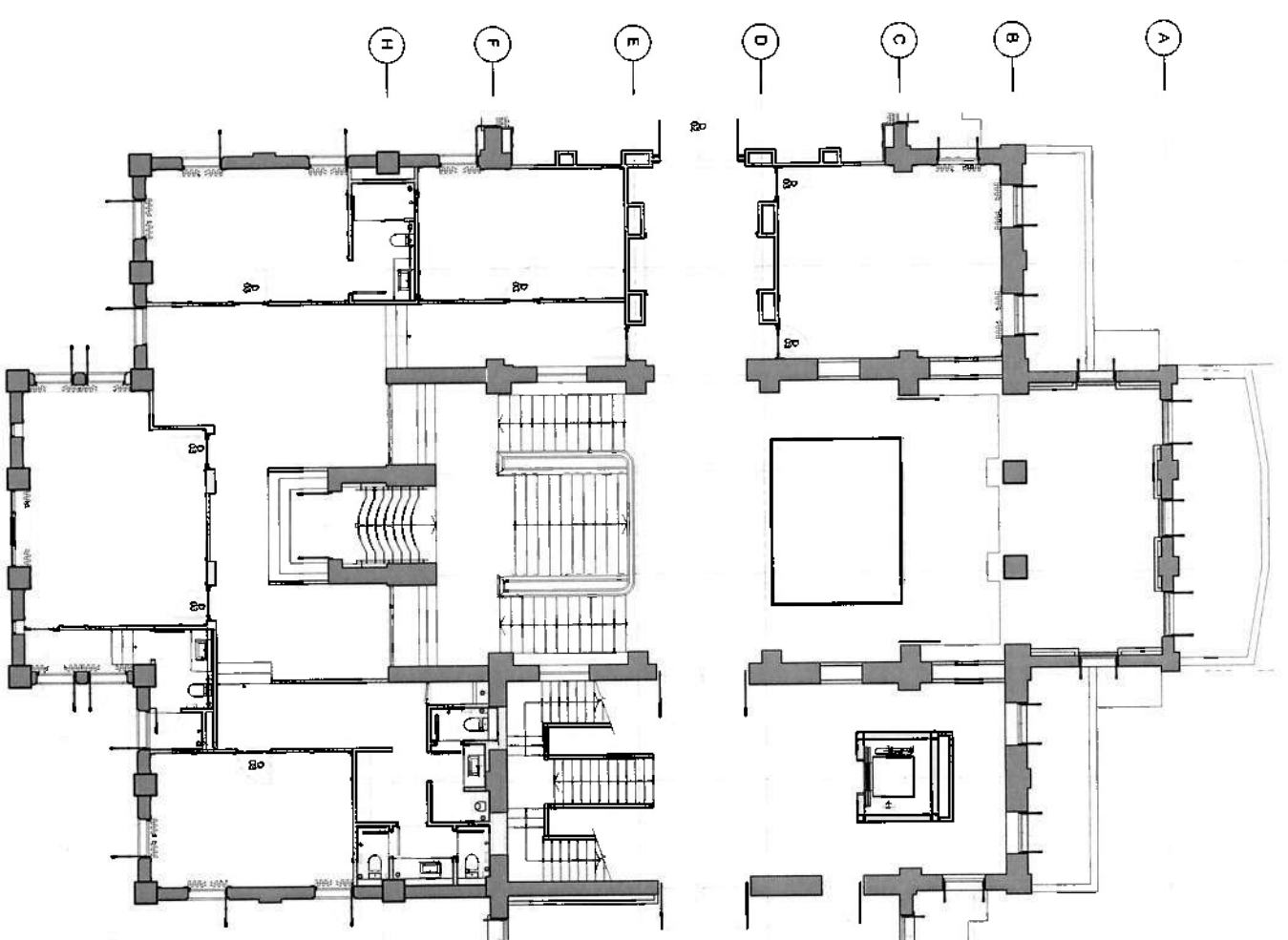
2nd FLOOR DOOR & WINDOW PLAN SCALE 1:100
