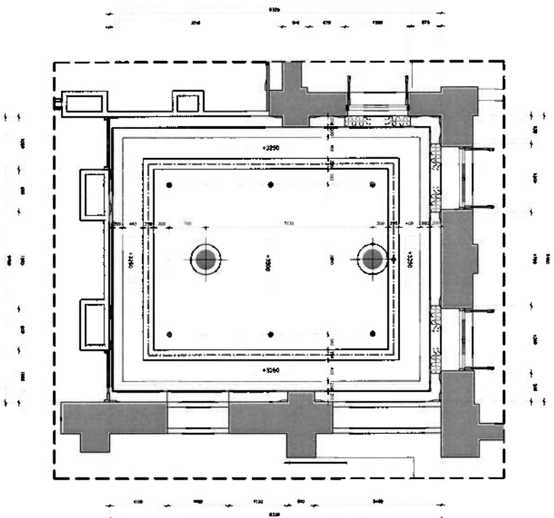
CEILING & LIGHTING LAYOUT SCALE 1:50
